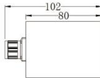
Unit: mm Dimension tolerance: ±2%
