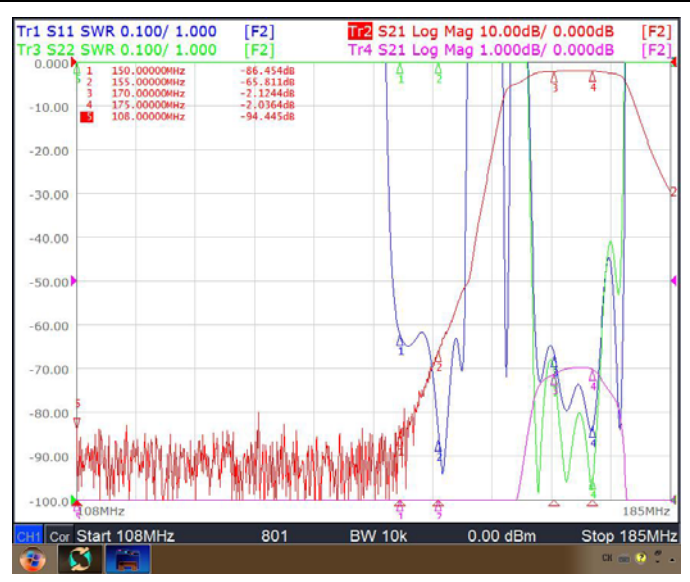
ANT-RX
