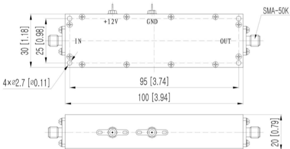
Outline drawing (unit: mm )
