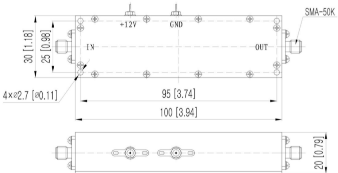
Outline drawing (unit: mm )
